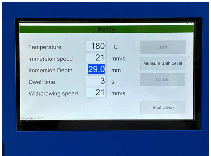
Touch panel display
